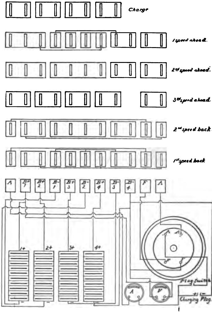
FIG. 303.—Diagram of Controller Connections of a Four-unit, One-motor, Circuit, with Constant Series Connections for Fields and Armature in Forward and Backward Speeds.
